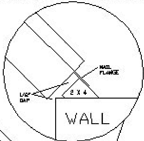
Nail Fin Installation Detail
